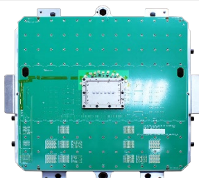
WLCSP Probe Card
