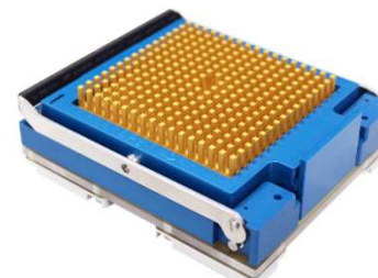
Burn-in Socket
