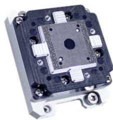
PoP Socket
